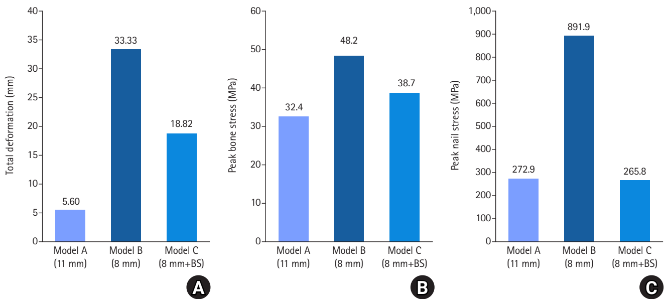
Fig. 6. Quantitative comparison of the three models. (A) Total deformation was 5.60, 33.33, and 18.82 mm in models A, B, and C, respectively. (B) Peak bone stress was 32.4, 48.2, and 38.7 MPa, respectively. (C) Peak nail stress was 272.9, 891.9, and 265.8 MPa, respectively. BS, blocking screws.
