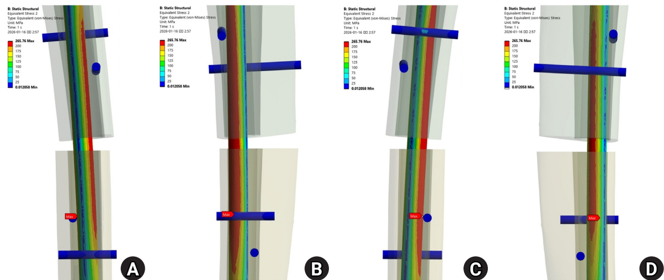
Fig. 5. Magnified distribution of von Mises stress around the defect in the model C nail. (A) Anterior, (B) medial, (C) posterior, and (D) lateral views are shown. The maximum nail stress was 265.8 MPa. Peak stresses in the individual blocking screws are reported in Table 3.
