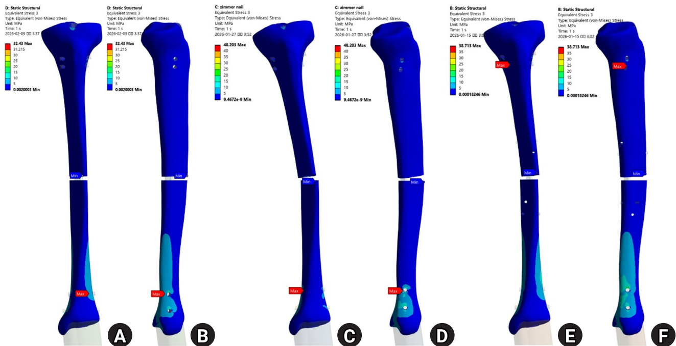
Fig. 3. Distribution of von Mises stress in the bone under axial loading, calculated across the entire bone domain. Peak bone stress was 32.4 MPa in model A (A, B), 48.2 MPa in model B (C, D), and 38.7 MPa in model C (E, F). Anterior views are shown in (A), (C), and (E), and medial views in (B), (D), and (F). Contour bands are identical across panels except for the uppermost band, which extends to the model-specific maximum.
