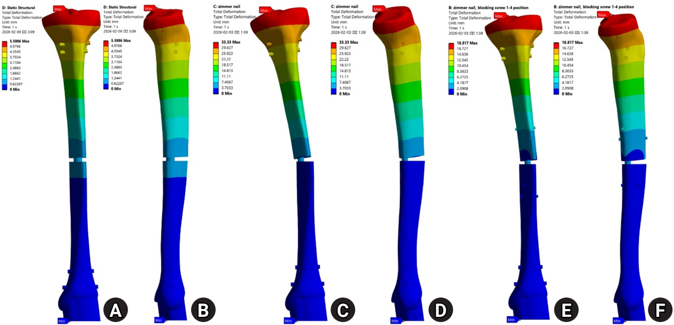
Fig. 2. Total deformation under axial loading. Maximum deformation was 5.60 mm in model A (A, B), 33.33 mm in model B (C, D), and 18.82 mm in model C (E, F) and occurred at the proximal tibia in all three models. Anterior views are shown in (A), (C), and (E), and medial views in (B), (D), and (F). The color scale was adjusted separately to the maximum value for each model; therefore, color differences between panels should not be interpreted as differences in absolute deformation.
