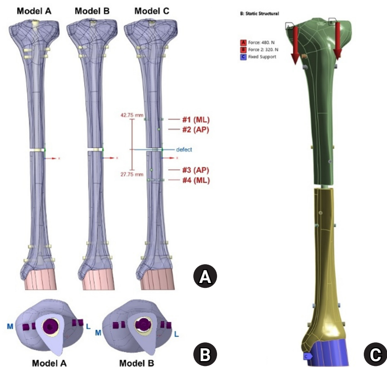
Fig. 1. Structural overview of the three finite element models. (A) Anterior views of model A, comprising an 11-mm nail with interlocking screws; model B, comprising an 8-mm nail with interlocking screws; and model C, comprising an 8-mm nail with four blocking screws. In model C, the blocking screws are numbered 1–4 from proximal to distal, and their insertion directions are indicated. Screws 1 and 4 are positioned 42.75 mm from the margin of the defect, and screws 2 and 3 are positioned 27.75 mm, measured to the screw axis. (B) Axial cross-sections of models A and B at the level of the defect, corresponding to the medullary isthmus and viewed from distal to proximal. Cortical bone is shown in light violet, cancellous bone in pale yellow, and the implants in magenta. The screws visible in these sections are interlocking screws. Model C is not shown because its nail is identical to that in model B and its blocking screws lie outside the illustrated plane. (C) Loading configuration consisting of an 800-N static axial load—480 N medially and 320 N laterally—and fixed support at the distal articular surface. ML, mediolateral; AP, anteroposterior; L, lateral; M, medial.
