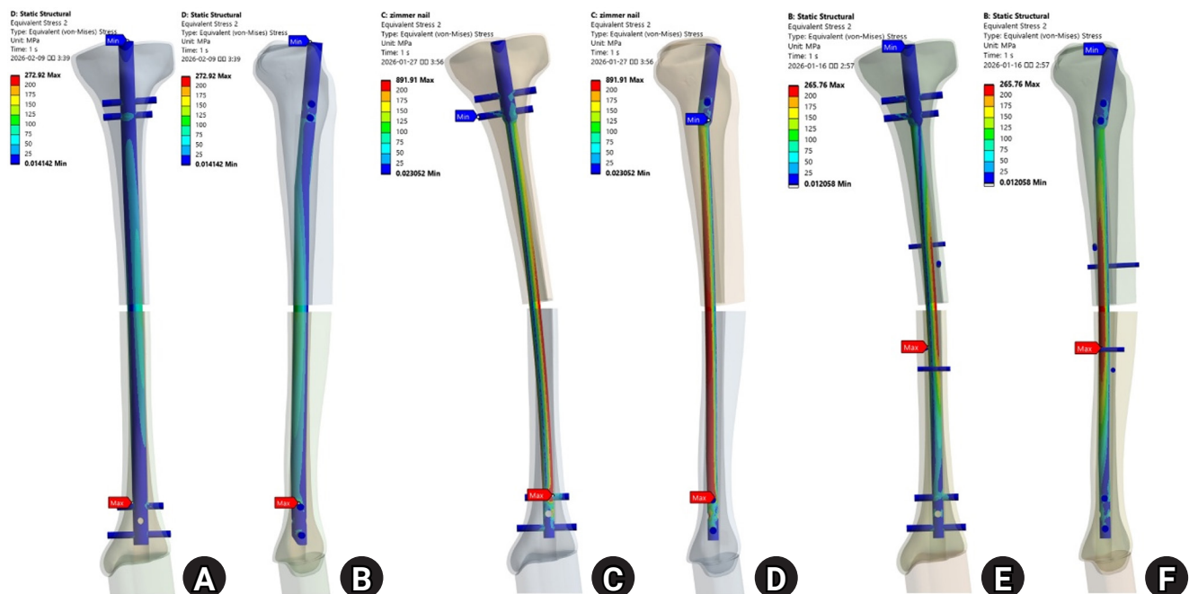
Fig. 4. Distribution of von Mises stress in the nail under axial loading. Peak nail stress was 272.9 MPa in model A (A, B), 891.9 MPa in model B (C, D), and 265.8 MPa in model C (E, F). Anterior views are shown in (A), (C), and (E), and medial views in (B), (D), and (F). Model B shows regions of elevated stress along the nail at the defect level, whereas the peak stress magnitude in model C is comparable to that in model A, although in model C the peak occurs at the level of the blocking screws. Contour bands are identical across panels except for the uppermost band, which extends to the model-specific maximum.
