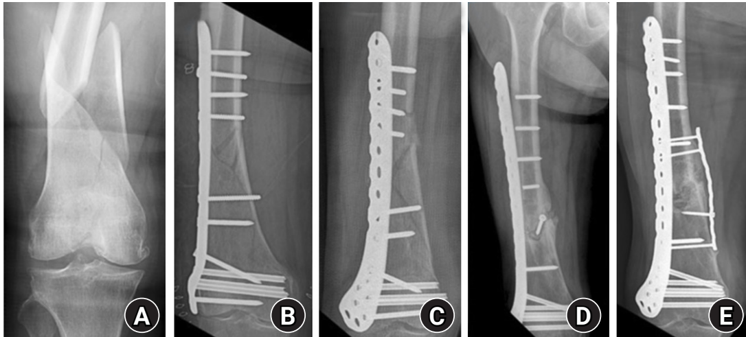
Fig. 7. (A) Radiograph of a 75-year-old female patient showing a spiral fracture with a butterfly fragment of the distal femur. (B) Lateral locked plating performed with two appositional screws at the fracture site. (C) Collapse of the fracture site with pull-out of the plate and proximal screws 2 months after surgery. (D) Additional fixation failure with breakage of the proximal screws after revision surgery using a longer locking plate. (E) Bony union achieved 9 months after the third operation, which included medial support plating and autologous iliac bone grafting.
